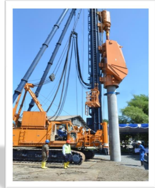
INNER-BORING: 5 INNER-BORING MACHINES
